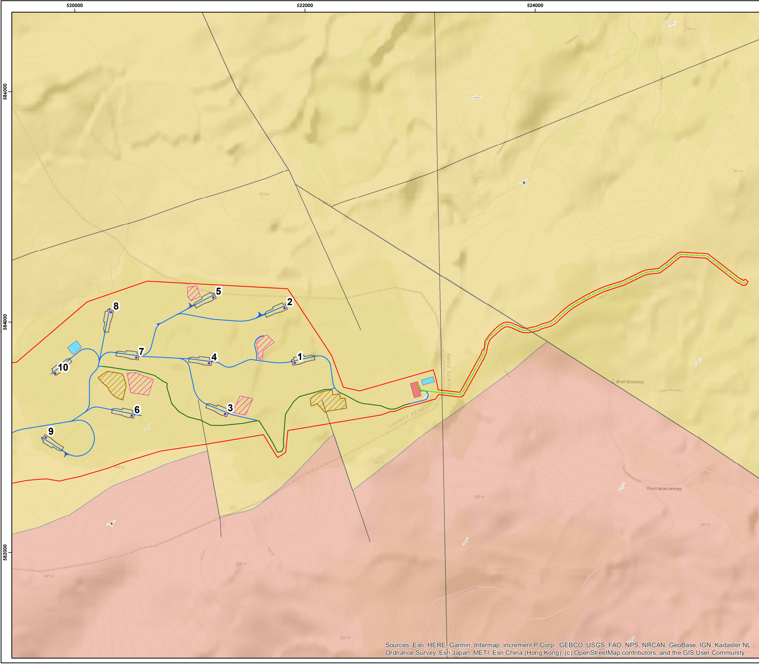
Figure10-3c Bedrock Geology
